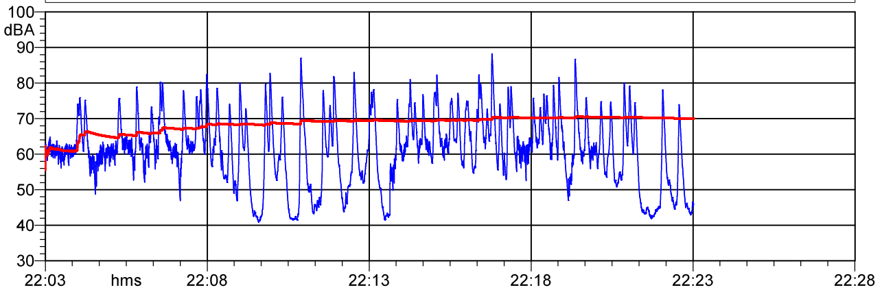
P4 - The Blossom - DD Alessandria LAeq - Running Leq
